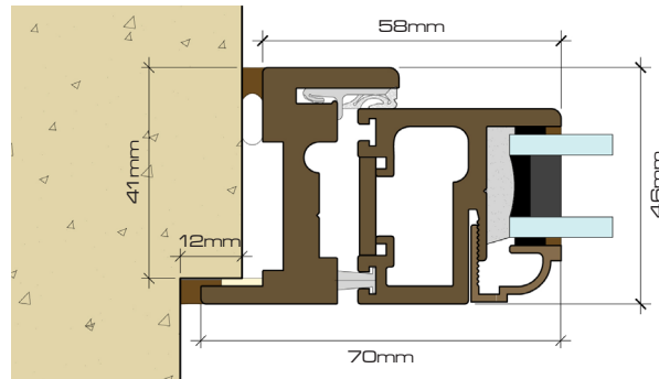
SECTION THROUGH SLIMLINE BRONZE DOORS
