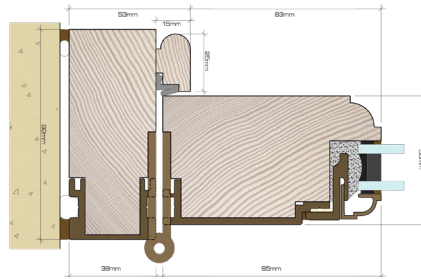
SECTION THROUGH BRONZE SINGLE CLAD DOOR SYSTEM
